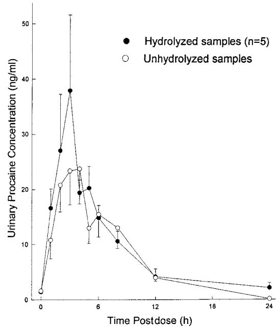
Fig. 4. Urinary procaine concentrations of hydrolyzed and unhydrolyzed samples following procaine HCl 5 mg SQ.
