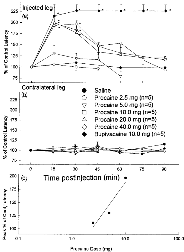
Fig. 3. (a) Hoof withdrawal reflex latency % increase following injection of procaine doses; (b) % change in contralateral leg following saline injection; (c) procaine dose-response curve. Asterisks indicate a significant difference from control values.
